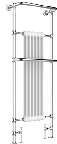
Grosvenor Size: 1500x 574 x 235 BTU: 2736 Pipe Center: 339mm Projection: 235mm Recommended Element: 400W Chrome GRO1500CW £730.00
