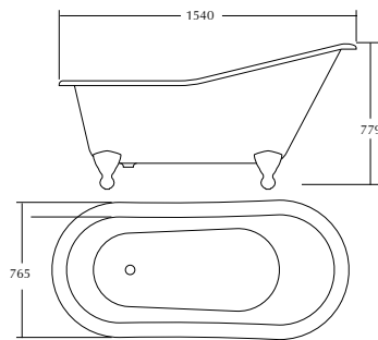
Ritz slipper bath - 1540 (Supplied with Imperial feet)
