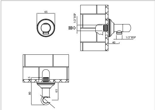
Hand shower kit (Suppled with a white handset) For use with the concealed shower valve
