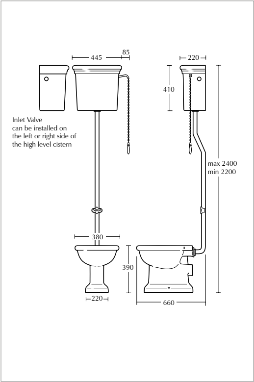
Ideal for use with P Trap pan: Ceramic connectors 236mm White XZ18070020 330mm White XZ18070010 Ceramic bend connector White XZ18070000 Plumber's mait - 750g For use with ceramic connectors PLUMB01
