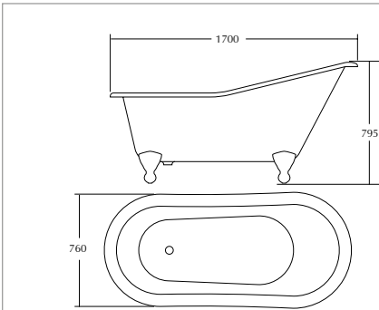
Ritz slipper bath - 1700 (Supplied with Imperial feet)
