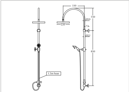
Edwardian rigid riser - slim Amena shower head (White handset) For use with the concealed shower valve
