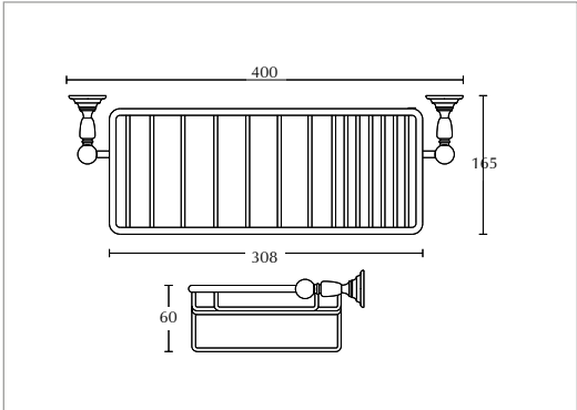
Richmond shower tidy wall mounted (For use with Victorian rigid riser kits)
