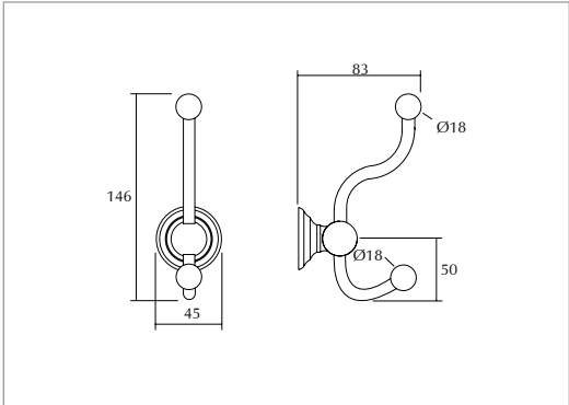
Double robe hook
