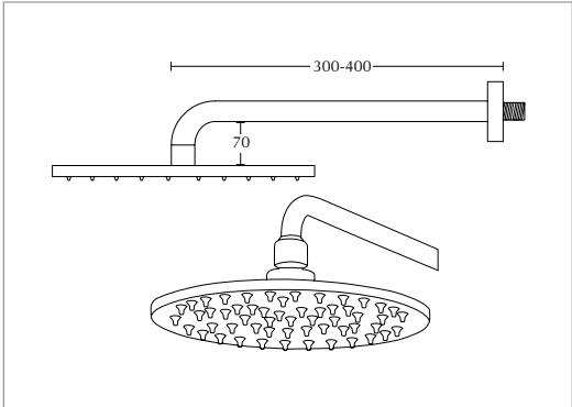
Amena Wall mounted slim rose head (Supplied with wall round fixed arm)
