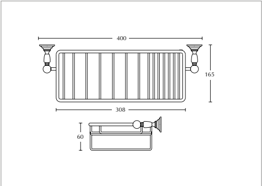
Richmond shower tidy wall mounted (For use with Victorian rigid riser kits) Chrome XCL0700100
