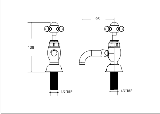
1/2" basin pillar taps White Cross Handle (finishes available with white cross handles) Chrome WESBASINTAPSWCP
