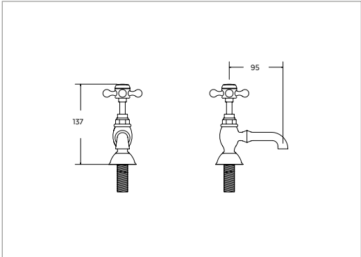
1/2" basin pillar taps
