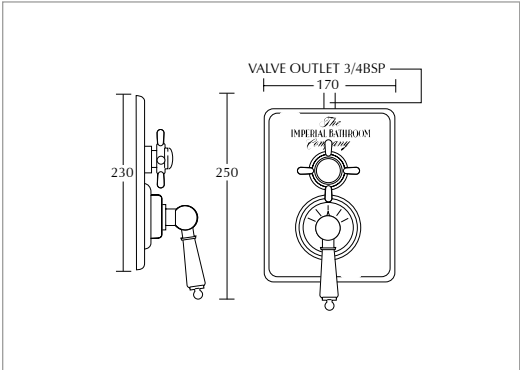
Concealed Victorian thermostatic dual control valve
