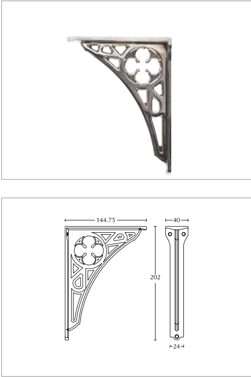
Ironbridge metal high level cistern brackets (Pair) Chrome XO18000030C Antique Gold XO18000030I Polished Nickel XO18000030N
