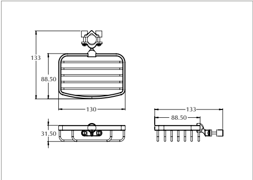
Victorian shower tidy soap rack (For use with Victorian and Westminster rigid riser kits) Chrome XS62800100N
