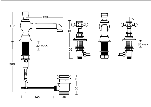
3 hole extended basin mixer 130mm (complete with pop up wastes)
