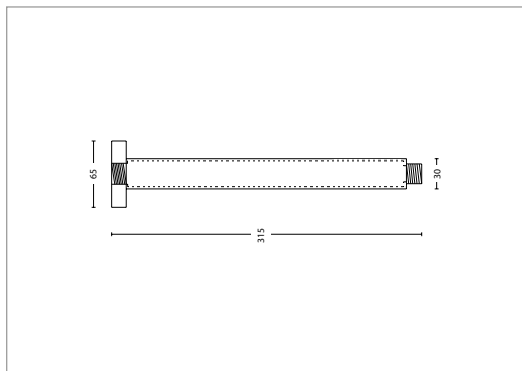
Ceiling shower adapter
