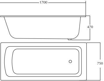
Harrington single ended cast iron bath (for use with Imperial bath panels)
