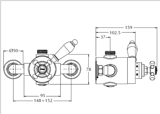
Exposed Westminster thermostatic control valve (Black controls) SINGLE WATER OUTLET Price for valve only
