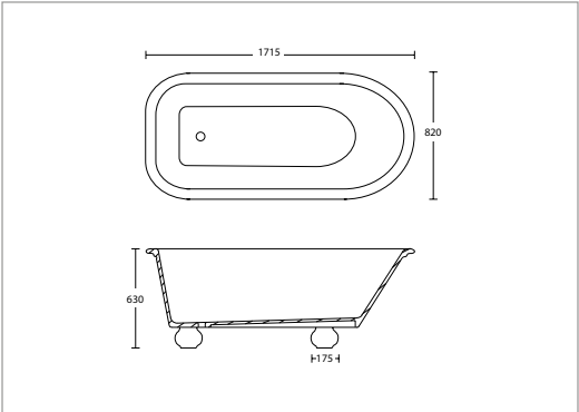
Stanlake Bath* supplied with ball feet
