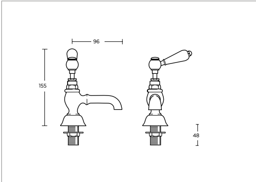
1/2" basin pillar taps White Ceramic Lever (finishes available with white ceramic levers) Chrome RADBASINTAPSWCP
