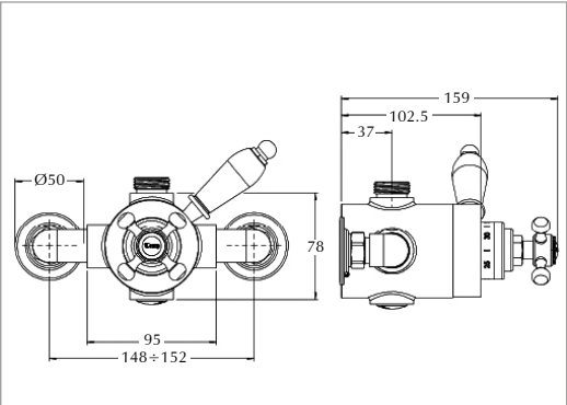
Exposed Westminster thermostatic control valve (White controls) SINGLE WATER OUTLET Price for valve only
